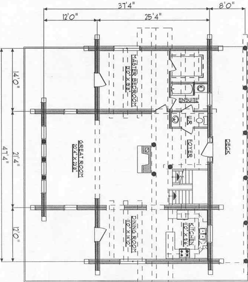
MAIN FLOOR PLAN 1575 SQ. FT.
